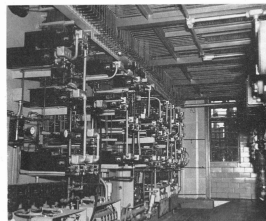
Here is a rear view of the graphic panel showing intricate piping layout which is necessary for air pressure instruments. No hydrocarbons enter the control room. All instrument impulses are transmitted to the board by pneumatic transmitters.
